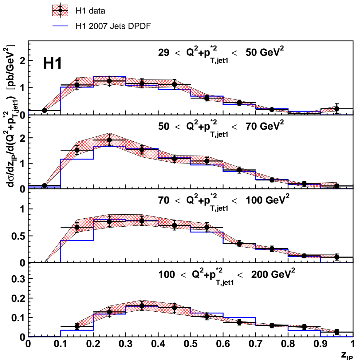
Figure 6: Cross section for diffractive dijet production doubly differential in z_P and the scale Q^2 + p_{T,jet1}^{*2} . The data are shown as black points with the inner and outer error bars denoting the statistical and quadratically added uncorrelated systematic uncertainties, respectively. The hatched band indicates the correlated systematic uncertainty. The solid line shows the NLO QCD prediction based on the H1 2007 Jets DPDF. Data points in the highest z_P bin were not included in the fit since the hadronisation corrections cannot be evaluated reliably.
