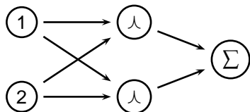
(c) RBF
