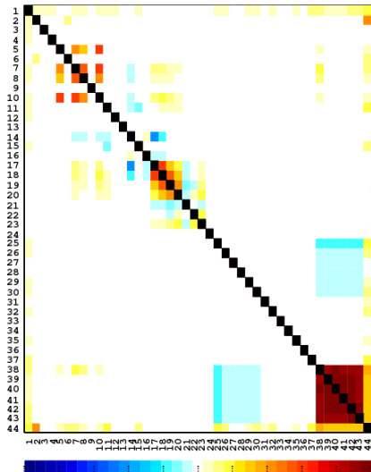
correlation matrix of input variables
